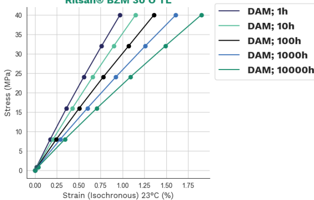
Stress-strain (Isochronous) 23°C Rilsan® BZM 30 0 TL
