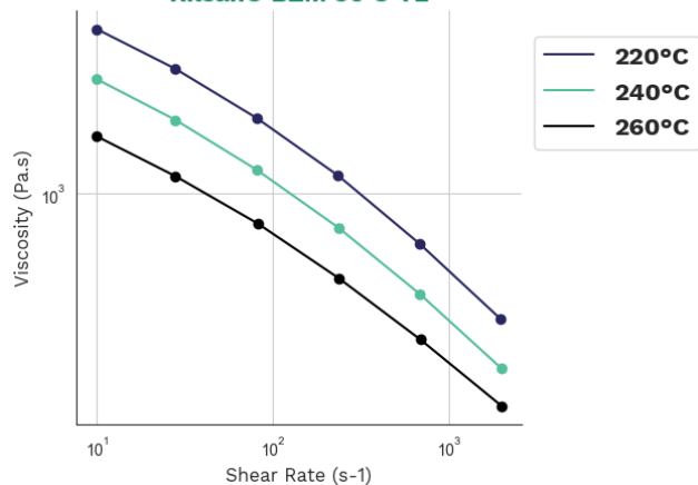
Viscosity-shear rate Rilsan® BZM 30 0 TL
