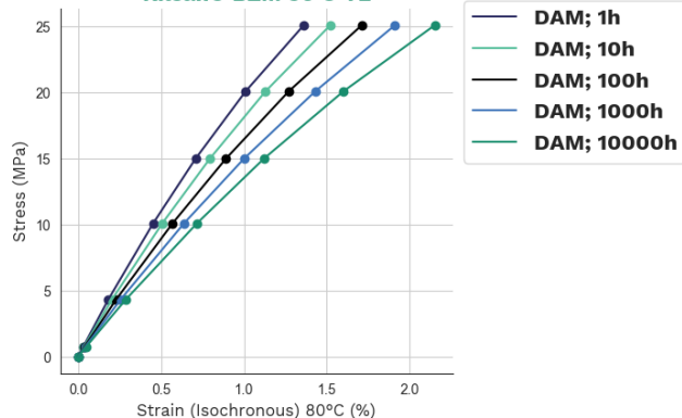
Stress-strain (Isochronous) 80°C Rilsan® BZM 30 0 TL
