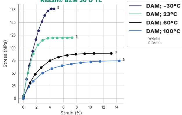
Stress-strain Rilsan® BZM 30 0 TL
